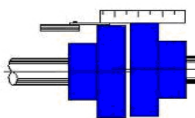
Figure 8. The straight edge and feeler gauge method of measuring Axial Alignment.
