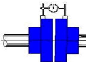
Figure 9. The preferred method of measuring Axial Parallelism.
