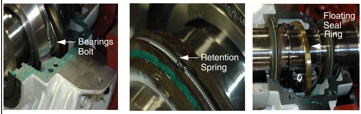
Figure 20. Drive End Bearing Removal.
