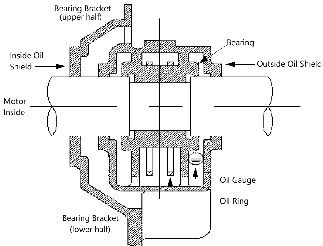
Figure 13. Oil Ring Lubricated Sleeve Bearings.
