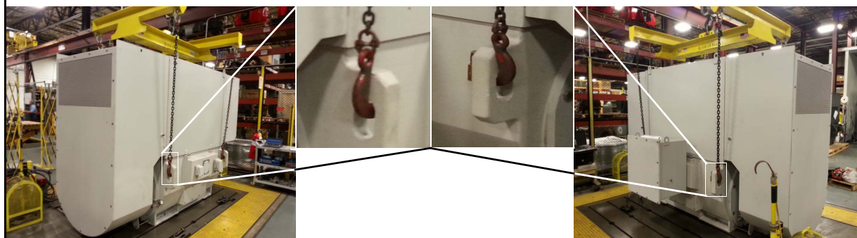
Figure 2. Typical lifting method used for large-scale motors.
