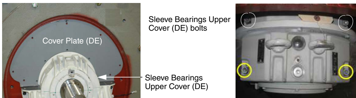
Figure 18. Assembly Covers for the Drive End Sleeve Bearings.
