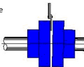
Figure 10. Feeler gauge method of measuring Axial Parallelism.
