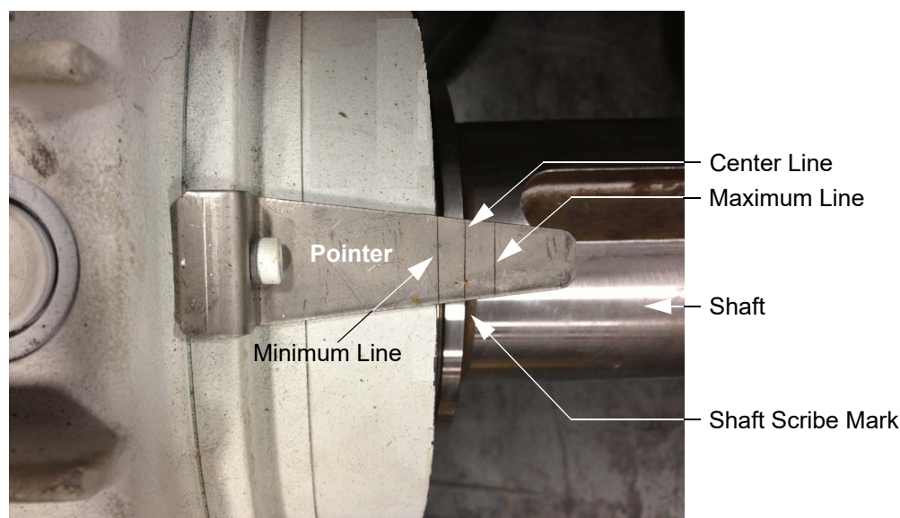
Figure 6. Magnetic Center Scribe Mark, Pointer, and Range.
