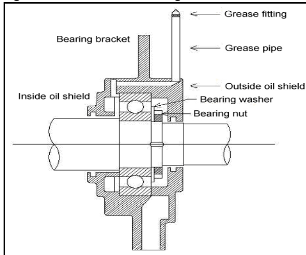
Figure 12. Antifriction Bearing Lubrication.
