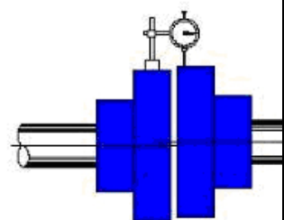
Figure 7. The preferred method of measuring Axial Alignment is with a dial indicator.
