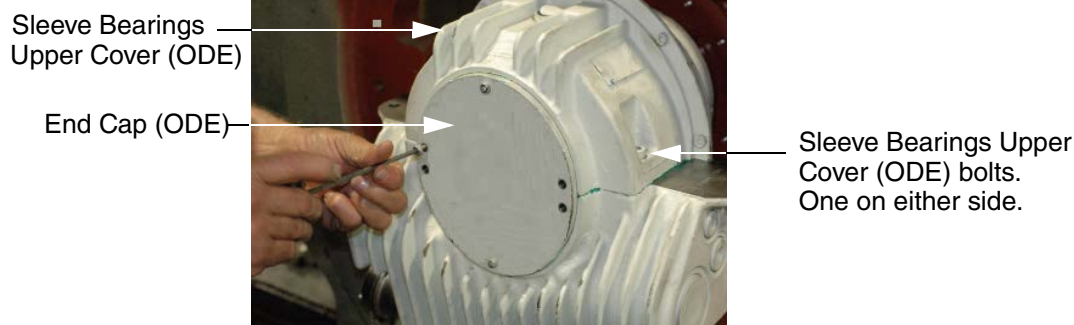
Figure 19. Opposite Drive End Sleeve Bearings Assembly.
