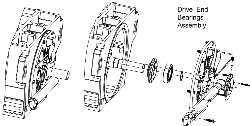
Figure 15. Drive End and Opposite Drive End Bearing Assemblies.
