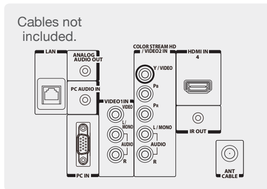
Rear Panel Connector Diagram
