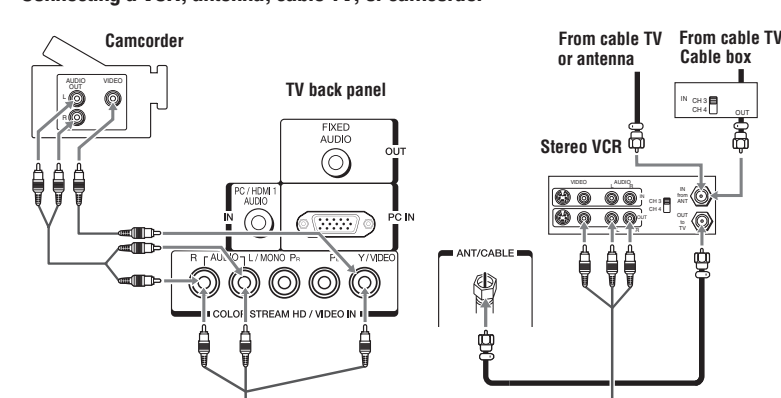
(Sample Illustration) Connecting to a VCR, antenna, or cable TV or camcorder
