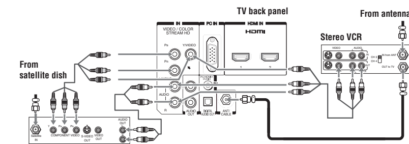
(Sample Illustration) Satellite receiver with component video or DVD player with component video
