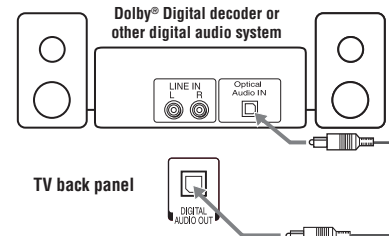
(Sample Illustration) Connecting a digital audio system
