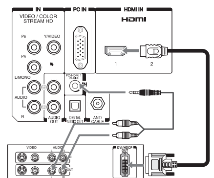
(Sample Illustration) DVI connections
