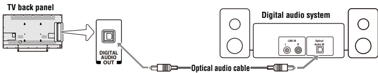
(Sample Illustration) L8400U Series—Connecting a digital audio system
