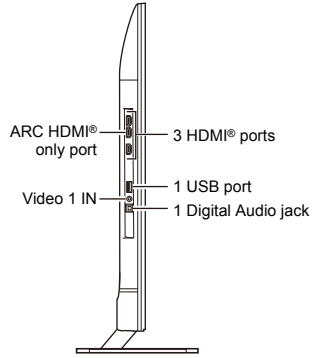
(Sample Illustration) L9400U Series—TV front and side panel controls
