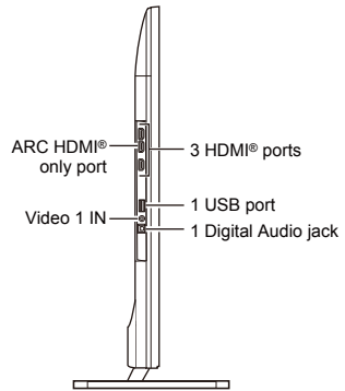
(Sample Illustration) L8400U Series—TV front and side panel controls
