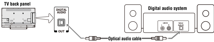
(Sample Illustration) L9400U Series—Connecting a digital audio system
