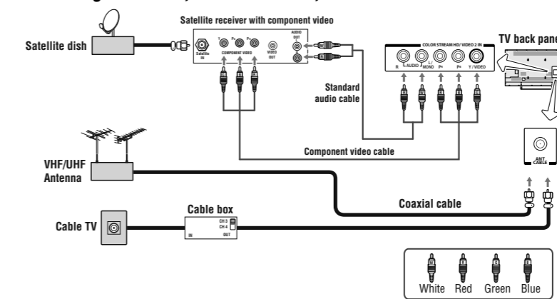
(Sample Illustration) Connecting to an antenna, satellite receiver, and cable TV box.
