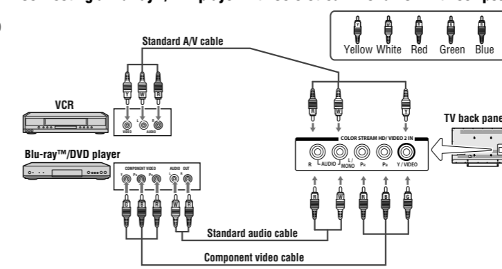
(Sample Illustration) Connecting a Blu-ray™ / DVD player with ColorStream™ or a VCR with composite video.
